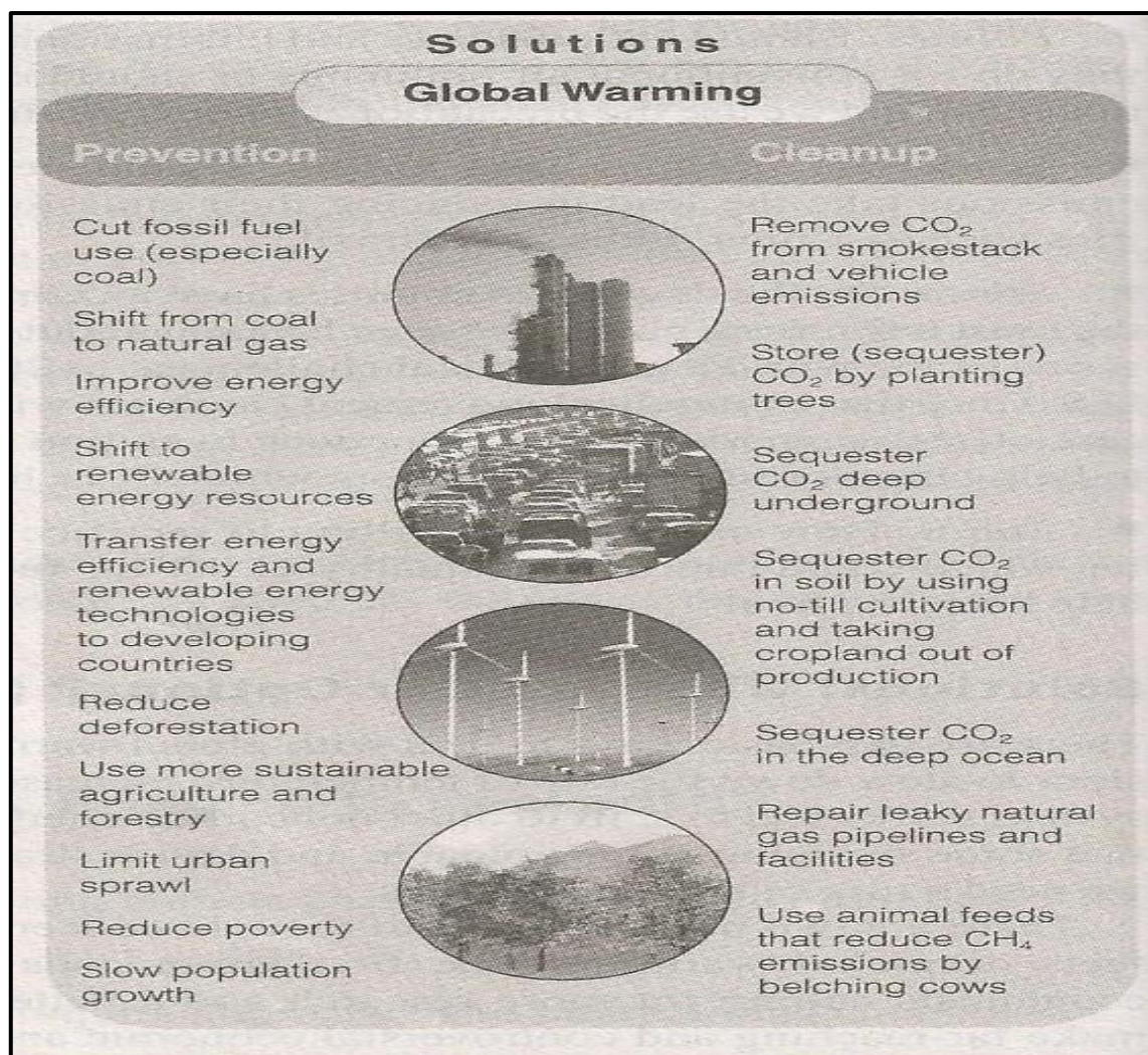
Figure 1.11 Solution to global warming
