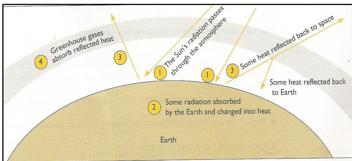
Figure 1.1 The greenhouse effect and global warming
